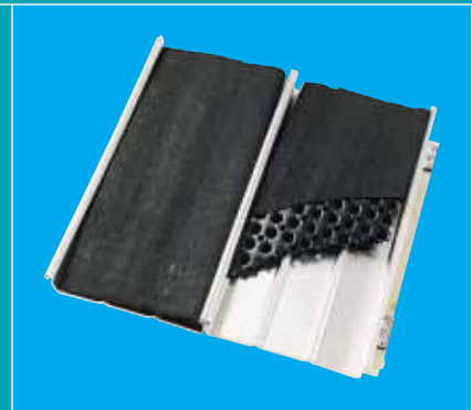
Drainage modular mat installed
